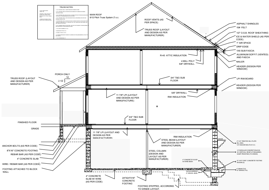
Two Story Full Section with Walkout
